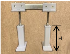
Low Profile Floor Mount Adjustable Pedestal MEP LP FLR-T2S Base 3" Wide – 3/8" Plate (Shown in Twin Configuration with U-Channel Bridge)
