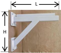
Wall Mount or Upright Braced HSS3x3 MEP WAL-T3S-I Base 8"x8" – 1/2" Plate
