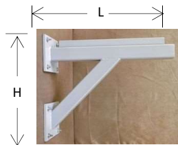
Wall Mount or Upright Braced HSS3x3 MEP WAL-T3S-L Base 8"x8" - 1/2" Plate
