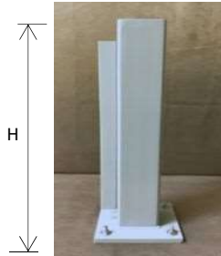
Upright Floor Mount Pedestal HSS4"x4", HSS 3"x3" MEP FLR-T4S Base 8"x8" - 1/2" Plate
